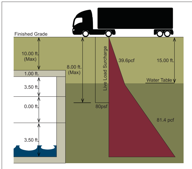
Figure 2. Lateral soil loads.
