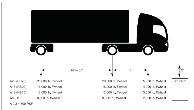
Figure 1. Vehicle load designations. ASTM C857-19.
