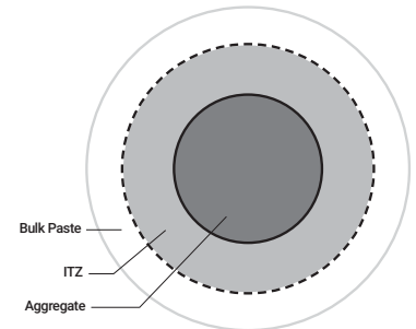
Figure 4: Aggregate ITZ
