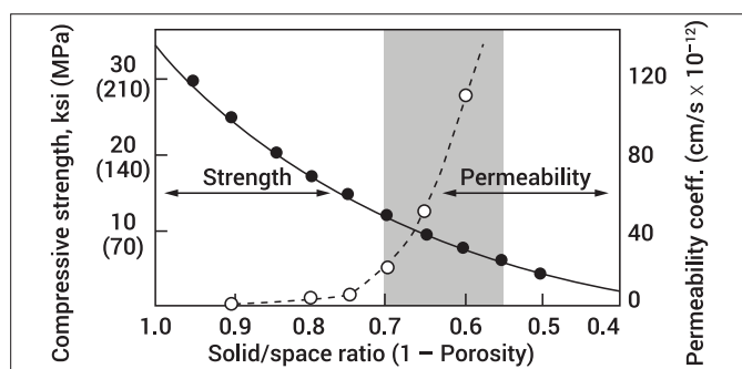
Figure 7: Graphical relationship between concrete porosity, strength and permeability. (Mehta and Monteiro, 1994) 1
