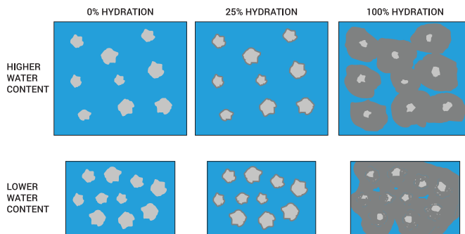
Figure 8: Influence of water content on cement grain spacing and porosity.
