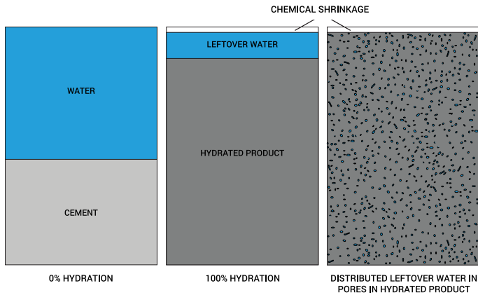
Figure 1: Water in concrete through different stages of hydration.
