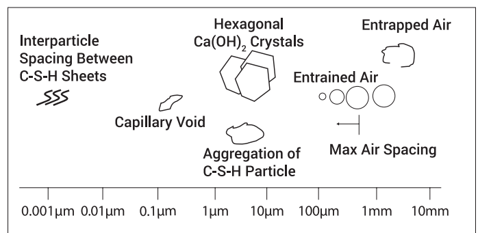
Figure 5: Range of sizes of pores in concrete.
