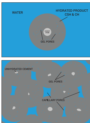
Figure 3: Formation of capillary pores as hydration occurs.
