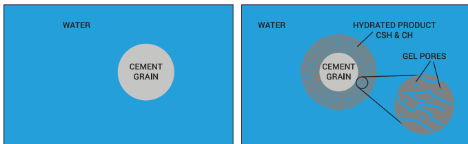
Figure 2: Formation of gel pores as hydration occurs.
