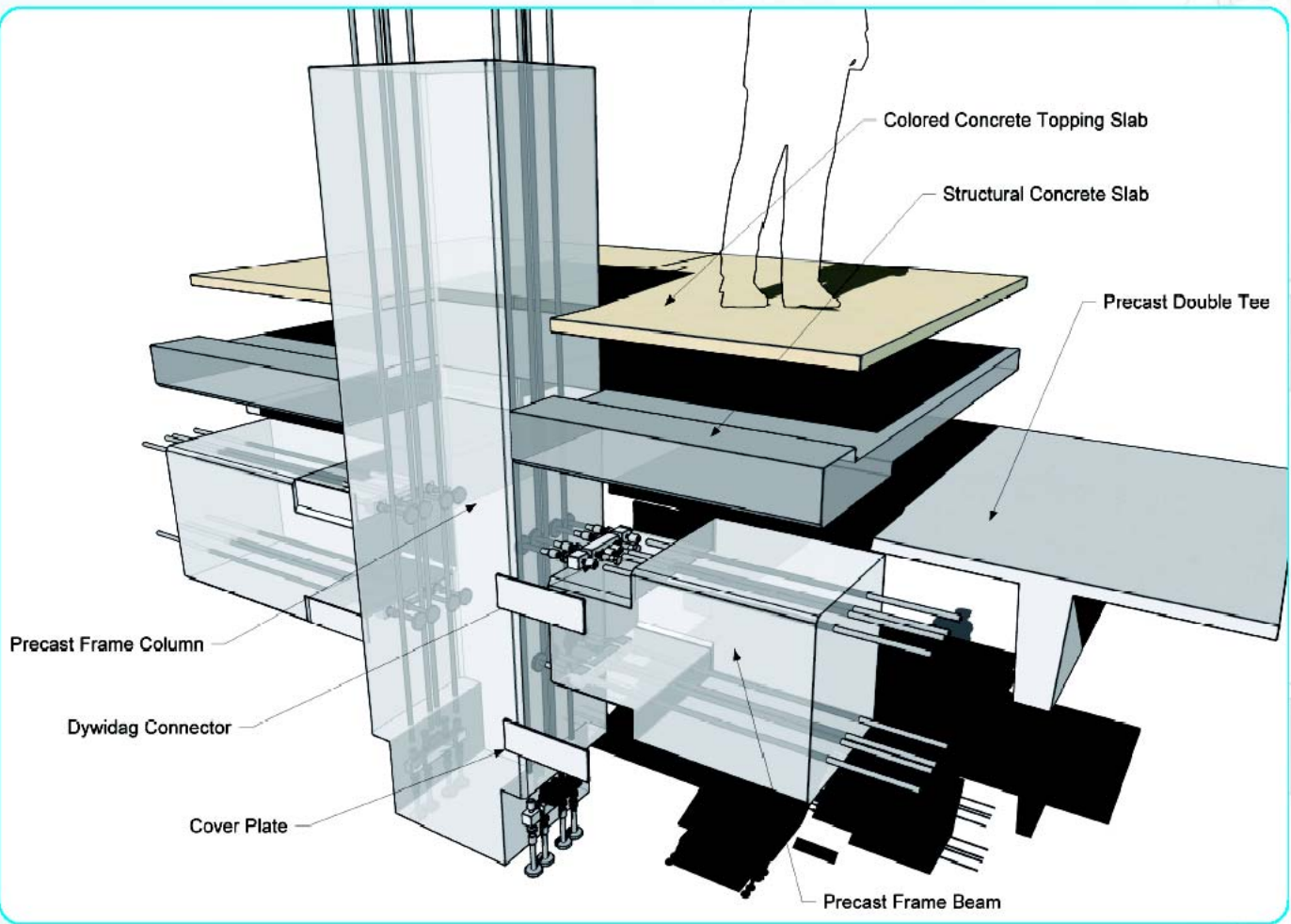
Exploded Detail Diagram of Precast Concrete Frame System and Concrete Deck Components.
